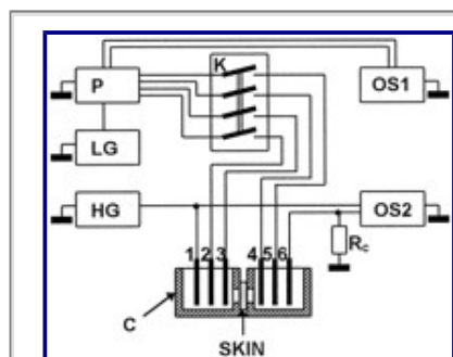
FIGURE 5 Schematic diagram of the experimental setup for skin capacitance and resistance measurements before, during, and after high-voltage electrotreatment. LG, low-voltage generator of triangular pulses; HG, high-voltage generator; PS, four-electrode potentiostat; C, cell with a skin sample and six (1-6) electrodes; OS1 and OS2, oscilloscopes.
