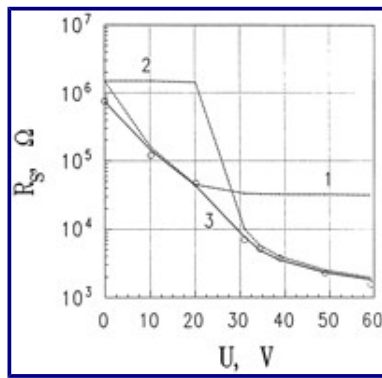
FIGURE 17 Skin resistance as function of voltage. Theoretical curves are for (1) appendageal pathway; (2) lipid-corneocyte pathway; (3) superposition of both pathways. \circ , experimental data have been obtained for skin sample with R_S^0 = 0.75 \text{ M}\Omega (see also Results for details). The following values of the parameters were used for pathway 2: \alpha_m = 0.02 \text{ V}^{-2} , R_t = 1.3 \text{ k}\Omega , G_m^0 = 6 \times 10^{-7} \Omega^{-1} , K_m = 5 \times 10^{-9} \Omega^{-1} \text{ s}^{-1} \text{ cm}^{-2} . For the appendageal pathway (1), all of the parameters are the same as in Fig. 16.
