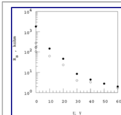
FIGURE 7 Voltage dependence of skin resistance R_s measured at 1 ms after the application of the pulse. \bullet and \circ correspond to the samples with different initial resistances R_S^O : \bullet , 1.8 M \Omega ; \circ , 100-300 k \Omega ; each open circle corresponds to the resistance averaged over five samples.
