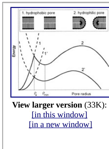
FIGURE 3 Energy of an electropore in a single lipid bilayer versus its radius. The hydrophobic (1) and hydrophilic (2) pores are displayed in the inset. The pore radius \rho^* corresponds to a structural rearrangement of the pore edge, and the hydrophobic pore is converted to a hydrophilic one. Pores accumulated in the local minimum \rho_{min} determine the electrical conductivity of the membrane. The electric field application (1' and 2' curves) reduces the potential barrier at \rho^* and, hence, increases pore population in the potential well \rho_{min} as well as the membrane conductivity.
