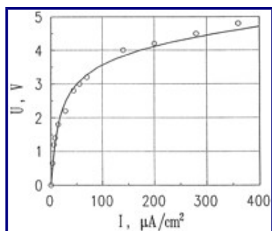
FIGURE 13 The comparison of theoretical (see Eqs. 11-14) current-voltage characteristic of skin sample (—) with experimental data (○) from Kasting and Bowman (1990) [1] . The values of the parameters (except \alpha_w = 0.4 \text{ V}^{-2} and h = 8.8 \times 10^{-3} \text{ cm} ) were the same as in Fig. 11.
