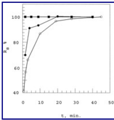
FIGURE 9 The recovery of skin sample resistance (in percent relative to the initial value) with R_S^0 = 75 \text{ k}\Omega after electrotreatment by single rectangular pulses of 8 ms duration and different amplitudes (in V): \circ , 50; \bullet , 35; \blacksquare , 10.
